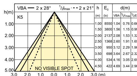
LDBE_CDMR111E_0009-Beam diagram
