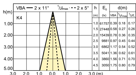
LDBE_CDMR111E_0007-Beam diagram
