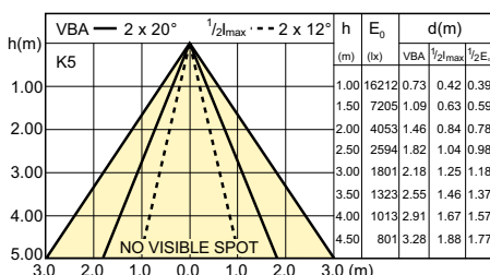
LDBE_CDMR111E_0008-Beam diagram
