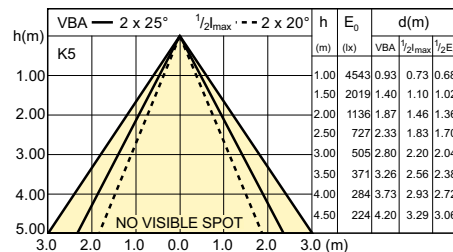
LDBE_CDMR111E_0003-Beam diagram
