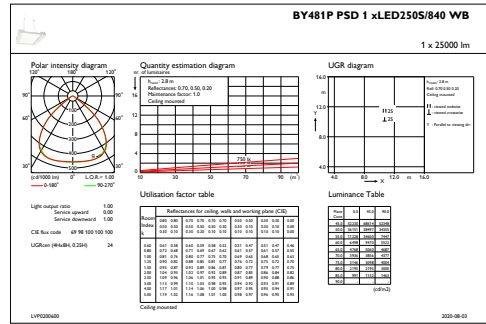
IFGU1_BY481PPSD1xLED250S840WB
