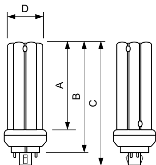
MASTER PL-T TOP 57W/840/4P 1CT/5X10BOX
