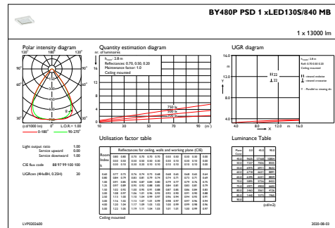
IFGU1_BY480PPSD1xLED130S840MB
