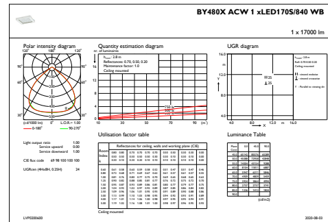
IFGU1_BY480XACW1xLED170S840WB
