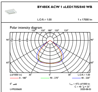
OFPC1_BY480XACW1xLED170S840WB
