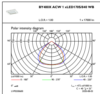
OFPC1_BY480XACW1xLED170S840WB
