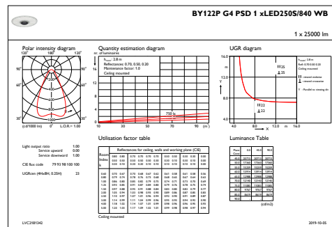
IFGU1_BY122PG4PSD1xLED250S840WB
