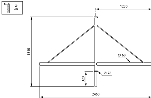
Caravelle brackets JRP322/323
